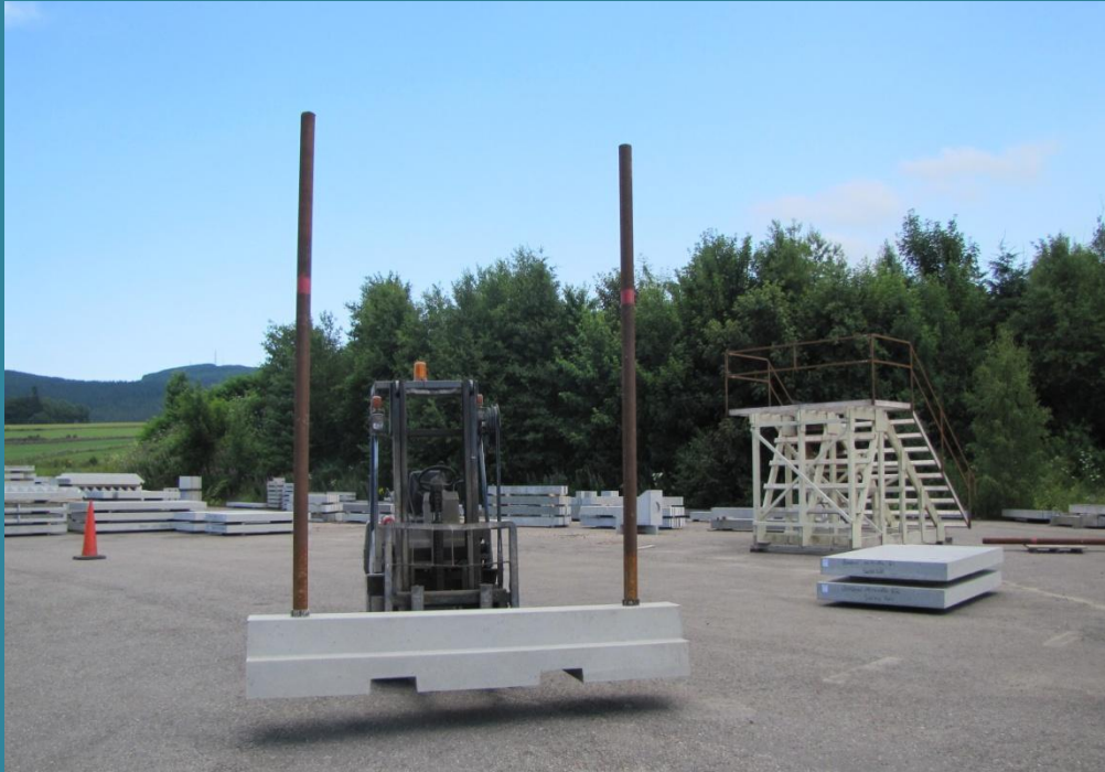
Rack with vertical pipe supports, movement by forklift
